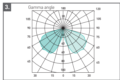
AL3921 150W SON-TD Mounting height: 5m
